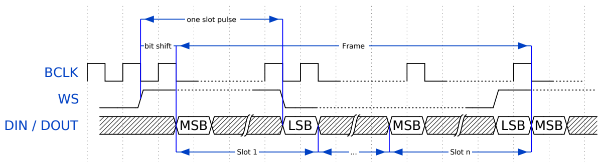
TDM PCM (long) Timing Diagram
