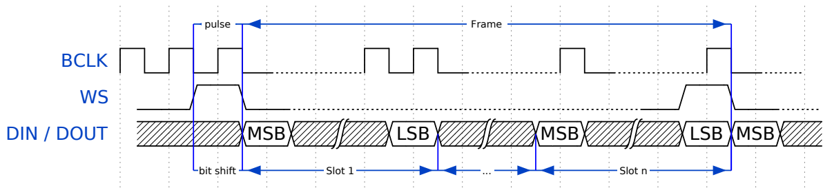
TDM PCM (short) Timing Diagram
