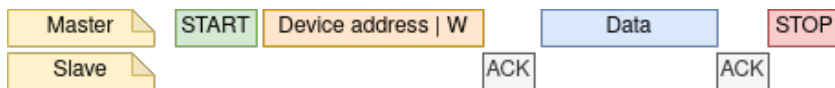
图 8: I2C master write to slave
