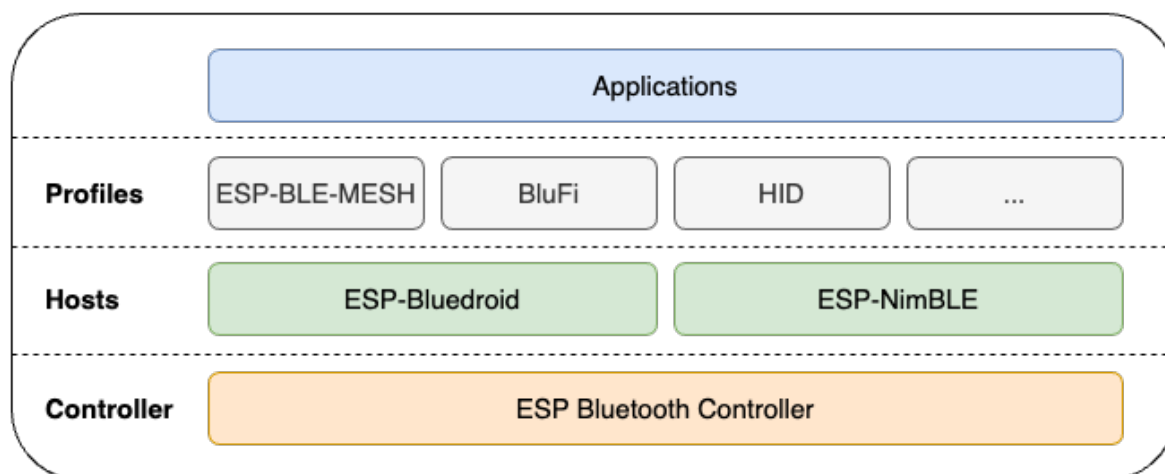
图 3: ESP32-C6 Bluetooth Stack Architecture
