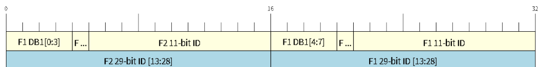
图 30: Bit layout of dual filter mode (Right side MSBit)
