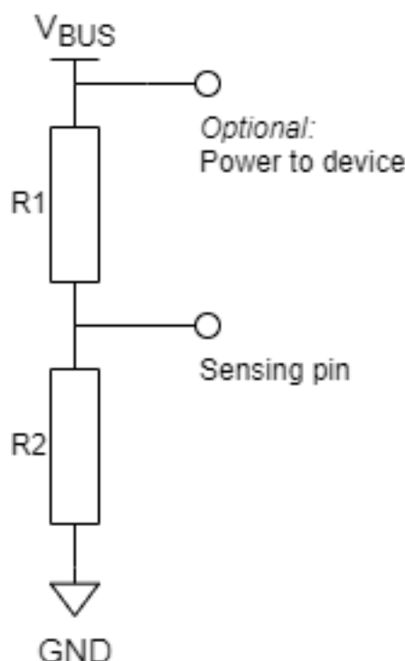
图 32: Simple voltage divider for VBUS monitoring
