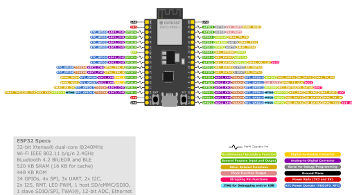
图 18: ESP32-DevKitM-1 (点击放大)
