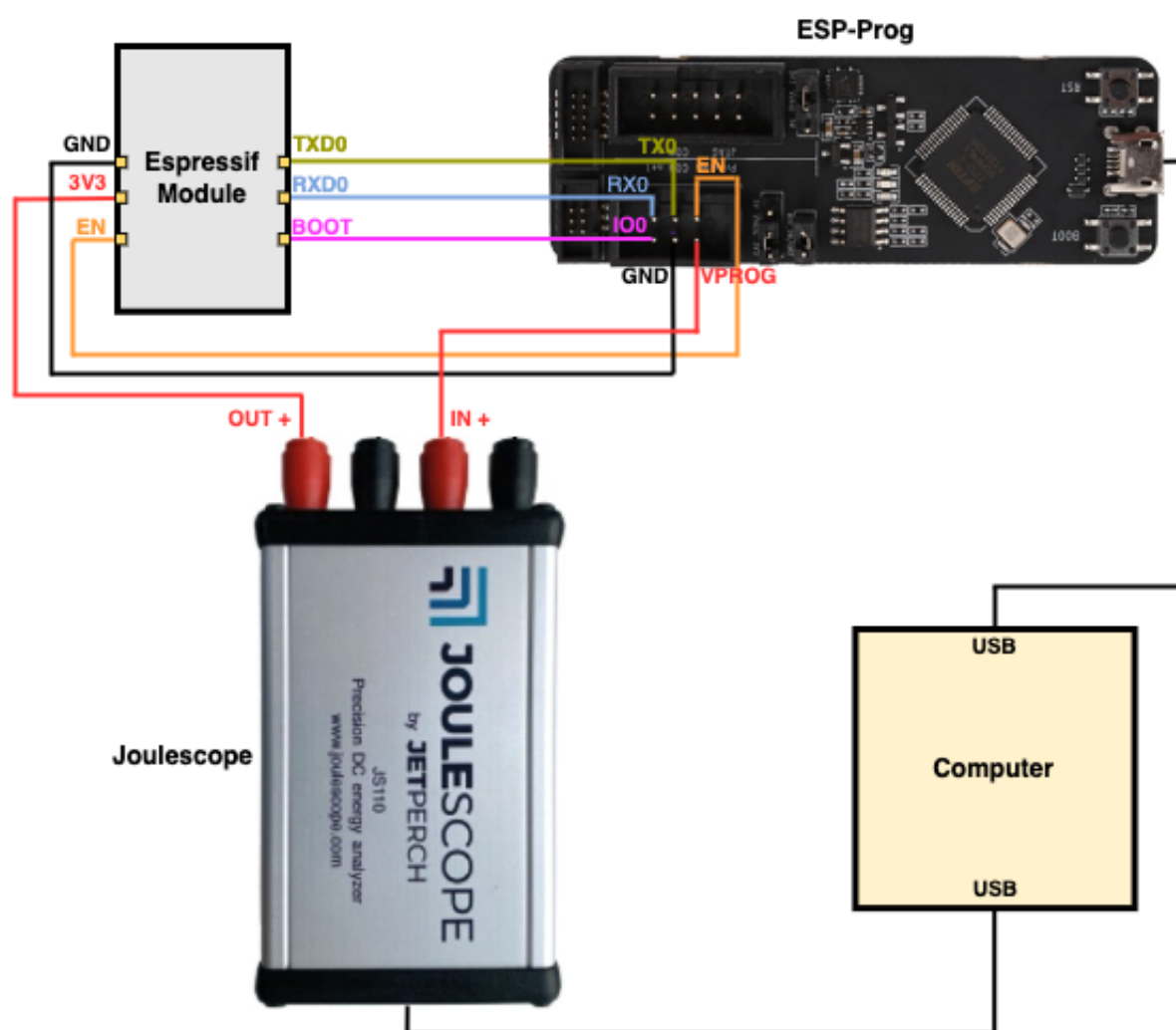
图 43: Hardware Connection (click to enlarge)
