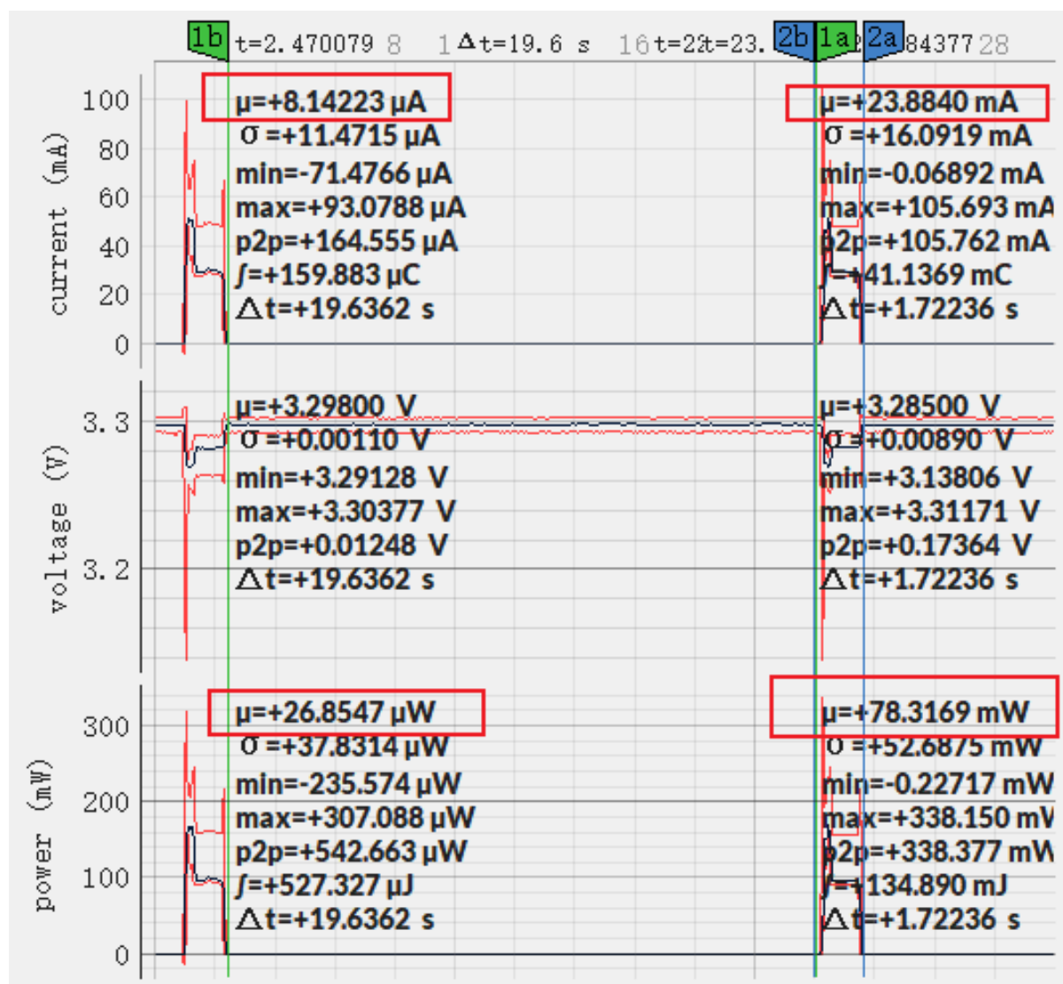
图 23: Current Waveform of ESP32-S3-WROOM-1 (click to enlarge)
