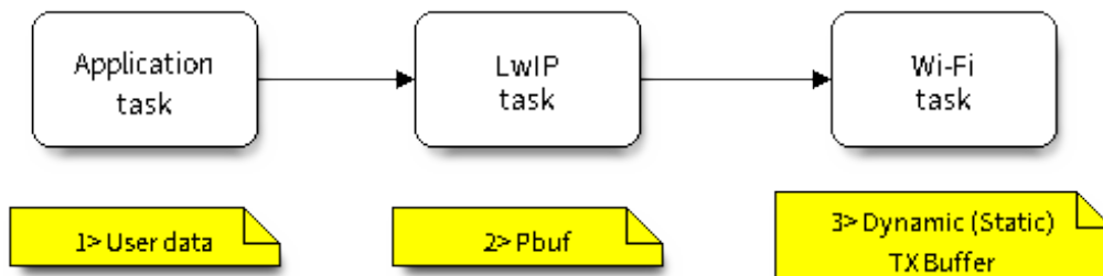
图 87: TX Buffer Allocation
