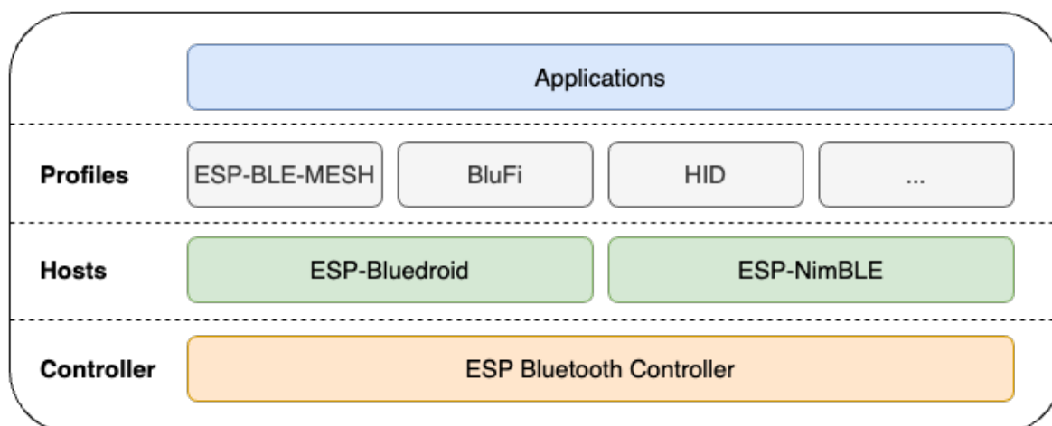
图 3: ESP32-C6 Bluetooth Stack Architecture
