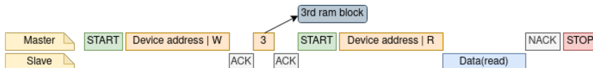
图 11: Get data from I2C slave RAM
