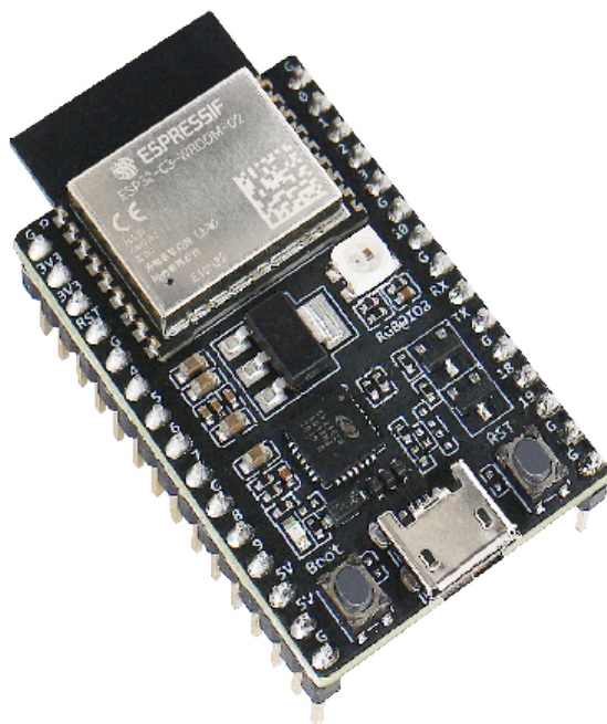
图 6: ESP32-C3-DevKitC-02
