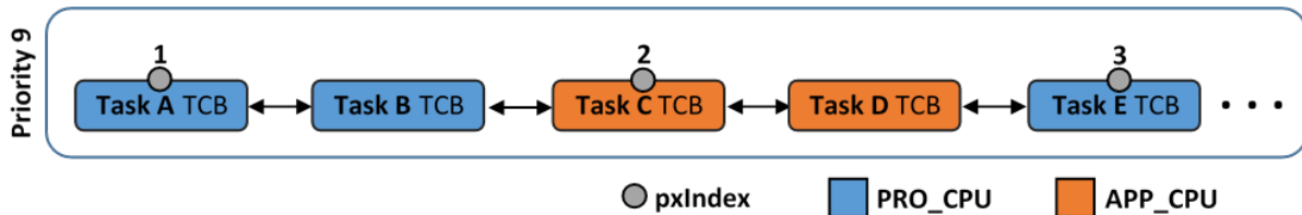
图 34: Illustration of pxIndex behavior in ESP-IDF FreeRTOS
