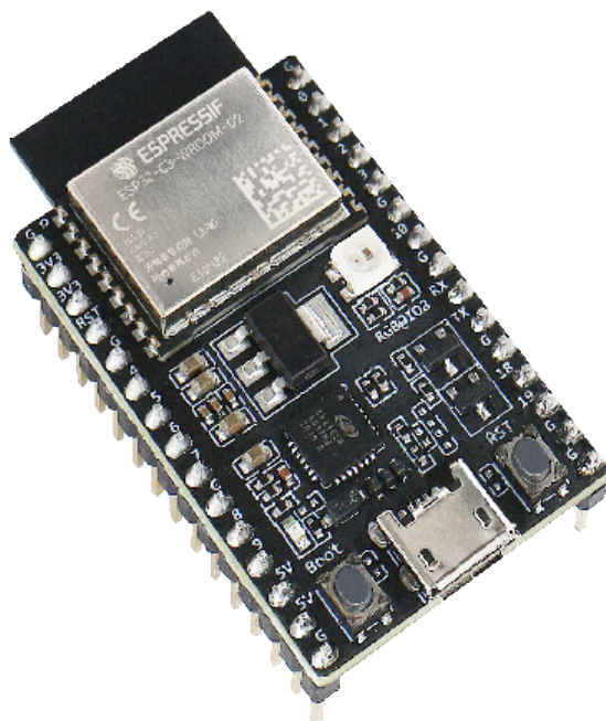
图 6: ESP32-C3-DevKitC-02
