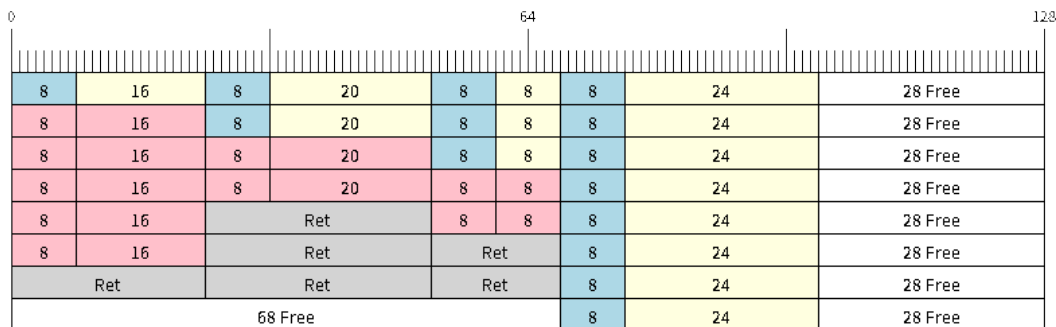
图 27: Retrieving/Returning items in No-Split and Allow-Split ring buffers
