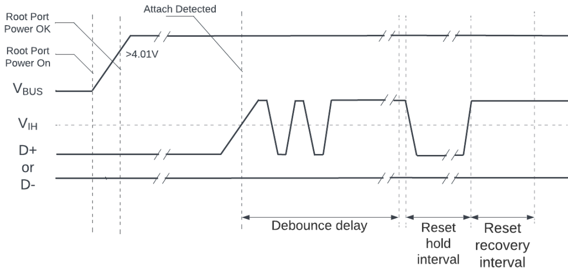
图 23: USB Root Hub Power-on and Connection Events Timing
