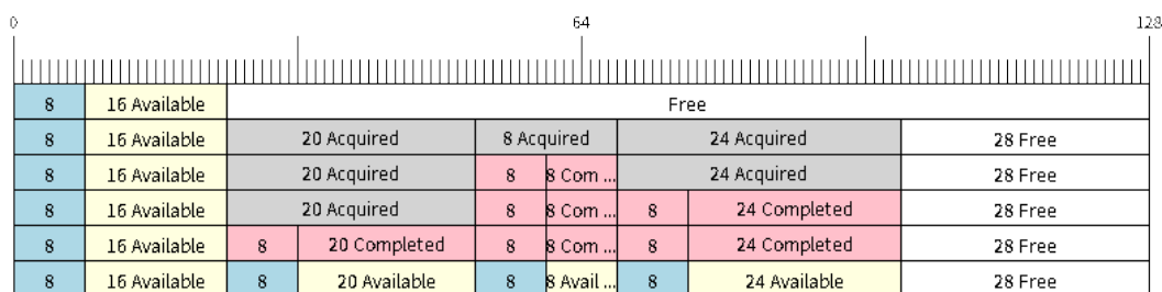
图 21: SendAcquire/SendComplete items in No-Split ring buffers
