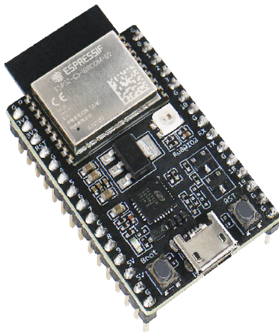
图 5: ESP32-C3-DevKitC-02
