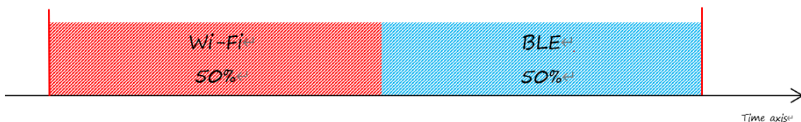
图 47: Wi-Fi CONNECTED 和 BLE CONNECTED 共存状态下时间片划分图
