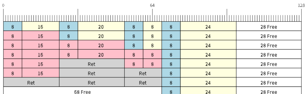
图 15: Retrieving/Returning items in No-Split and Allow-Split ring buffers
