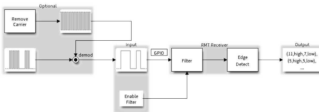
图 14: RMT Receiver Overview
