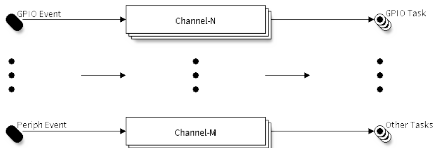
图 5: ETM channels Overview
