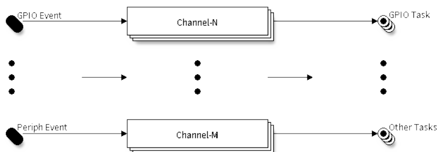
图 3: ETM channels Overview
