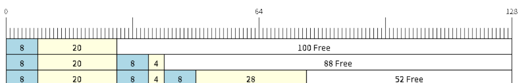
图 26: Sending items to No-Split or Allow-Split ring buffers
