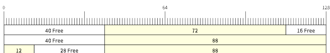
图 35: Wrap around in byte buffers
