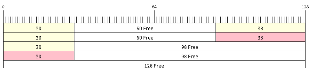
图 36: Retrieving/Returning items in No-Split and Allow-Split ring buffers
