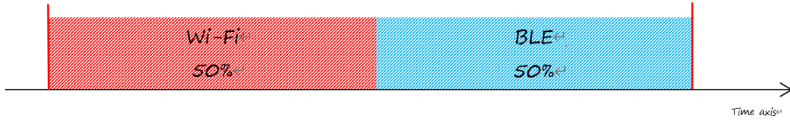
图 17: Wi-Fi CONNECTED 和 BLE CONNECTED 共存状态下时间片划分图
