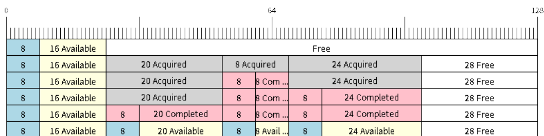
图 28: SendAcquire/SendComplete items in No-Split ring buffers
