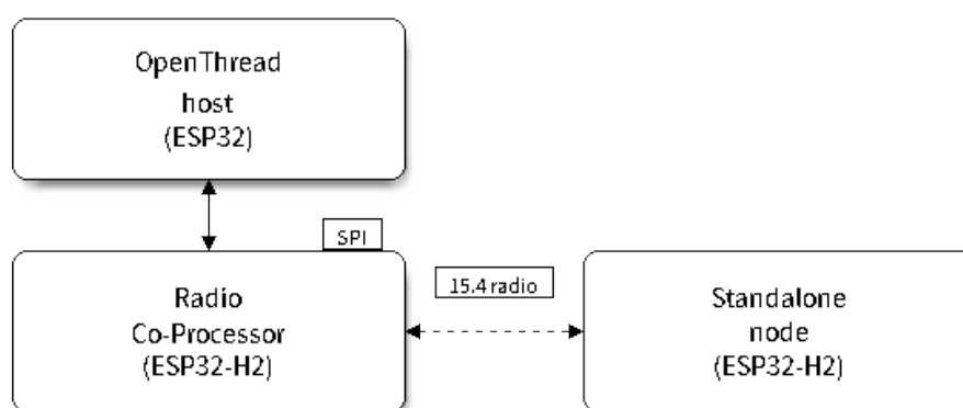
图 54: OpenThread device modes
