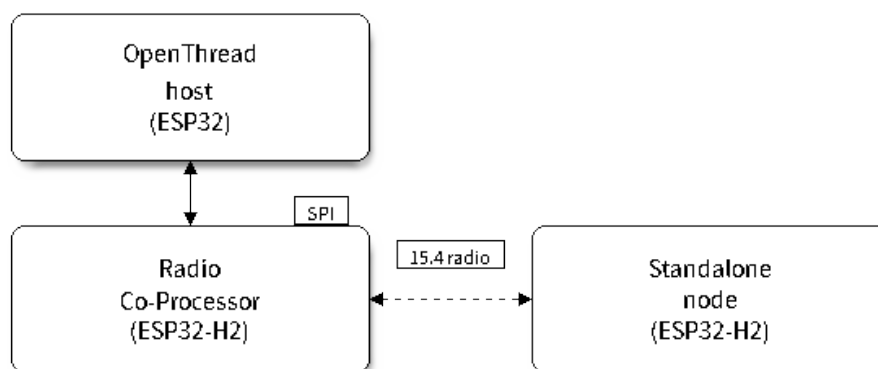
图 54: OpenThread device modes
