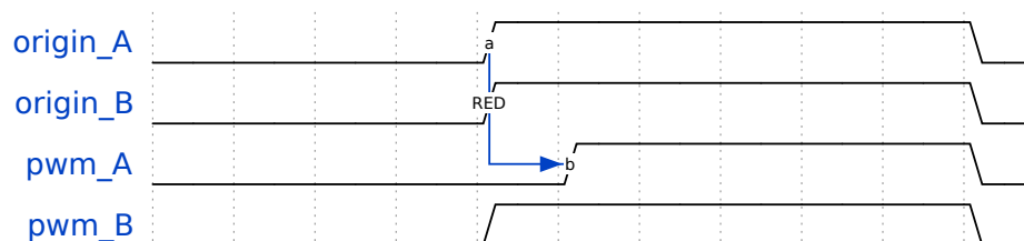
RED on A, Bypass B
