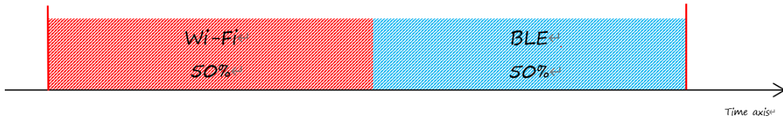
图 17: Wi-Fi CONNECTED 和 BLE CONNECTED 共存状态下时间片划分图
