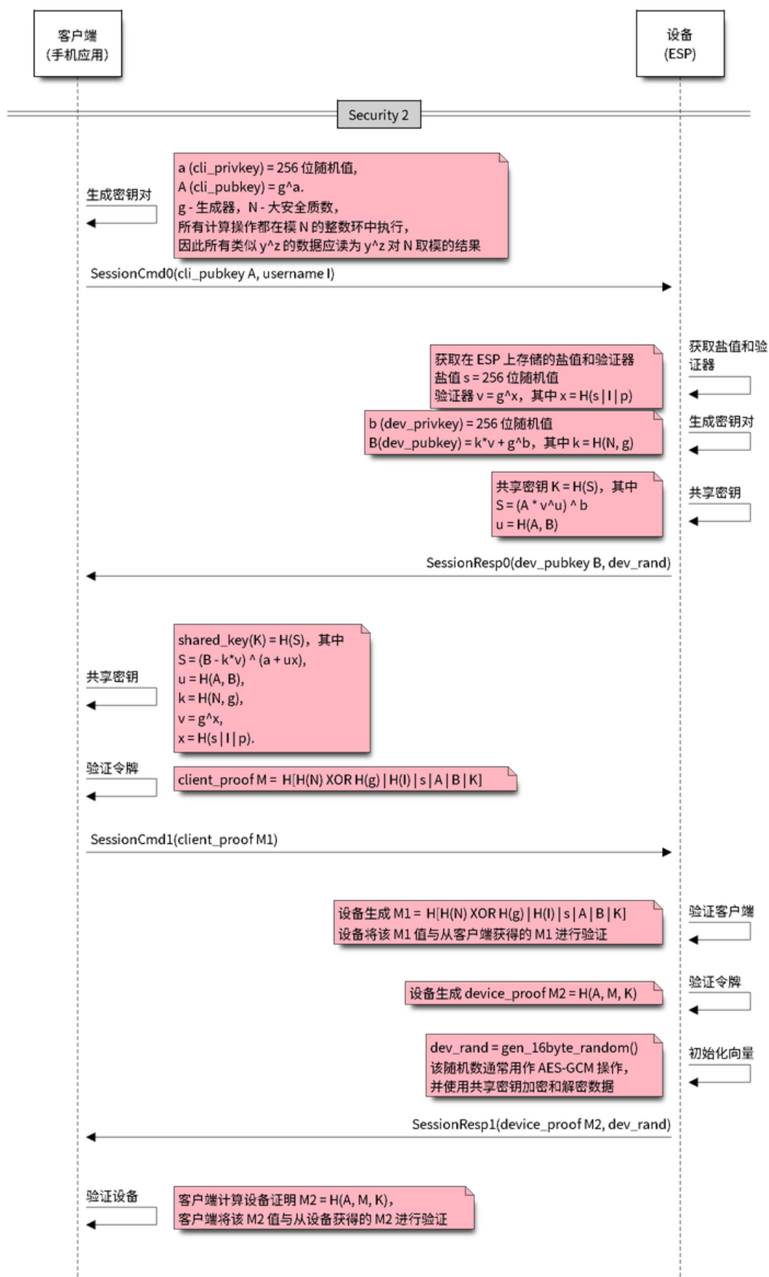
图 13: Security 2
