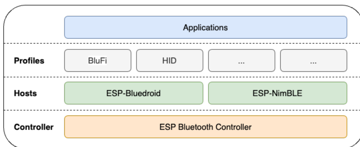
图 3: ESP32-C2 Bluetooth Stack Architecture
