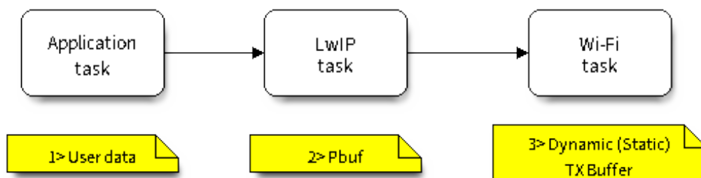
图 38: TX Buffer Allocation
