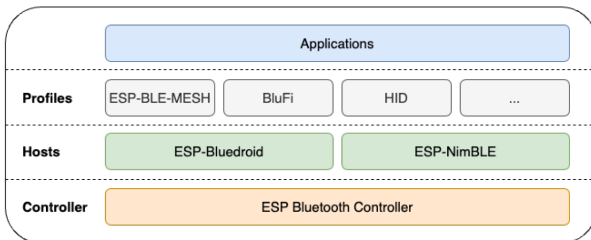
图 3: ESP32-C3 Bluetooth Stack Architecture
