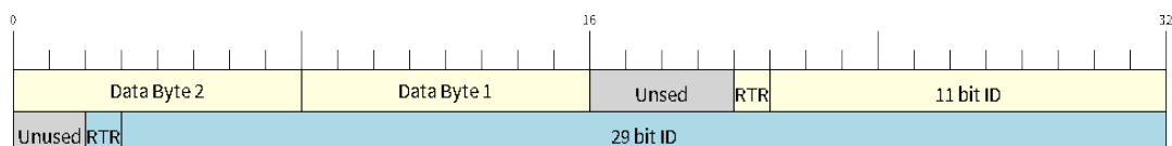
图 29: Bit layout of single filter mode (Right side MSBit)
