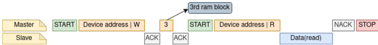
图 13: Get data from I2C slave RAM
