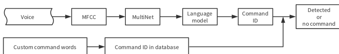
Fig. 1: speech_command-recognition-system
