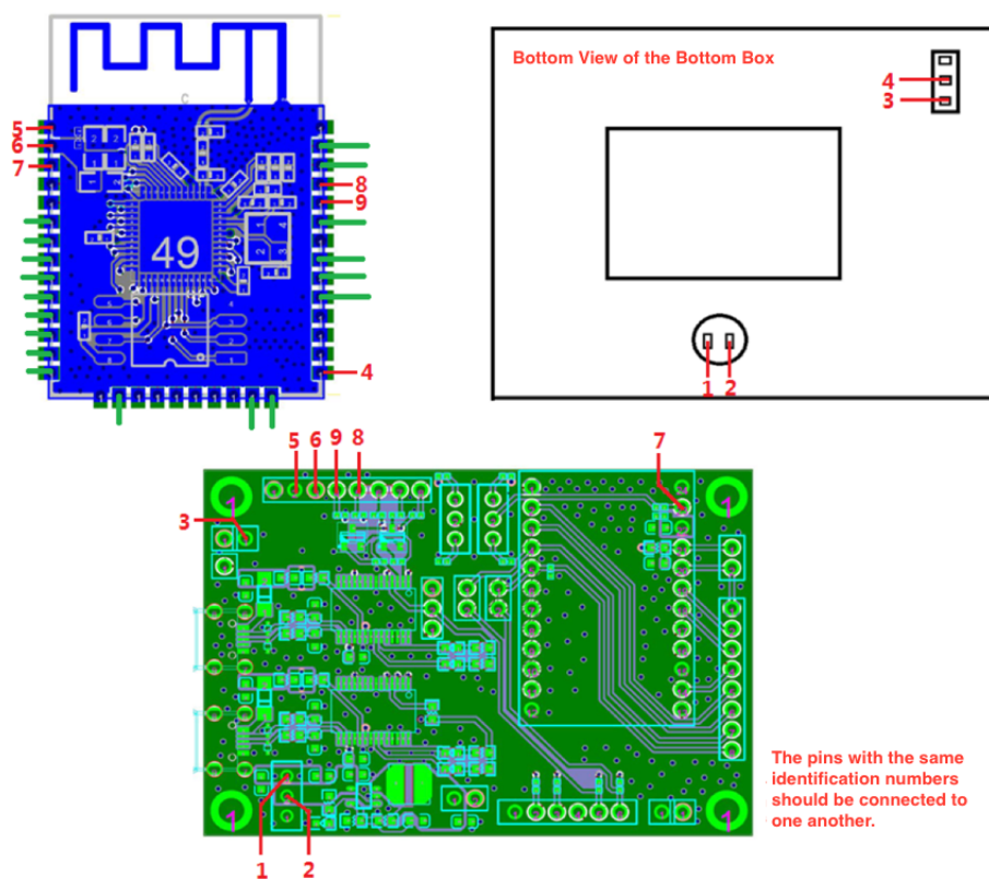
Fig. 95: The Wiring of the ESP32-WROOM-32 Fixture
