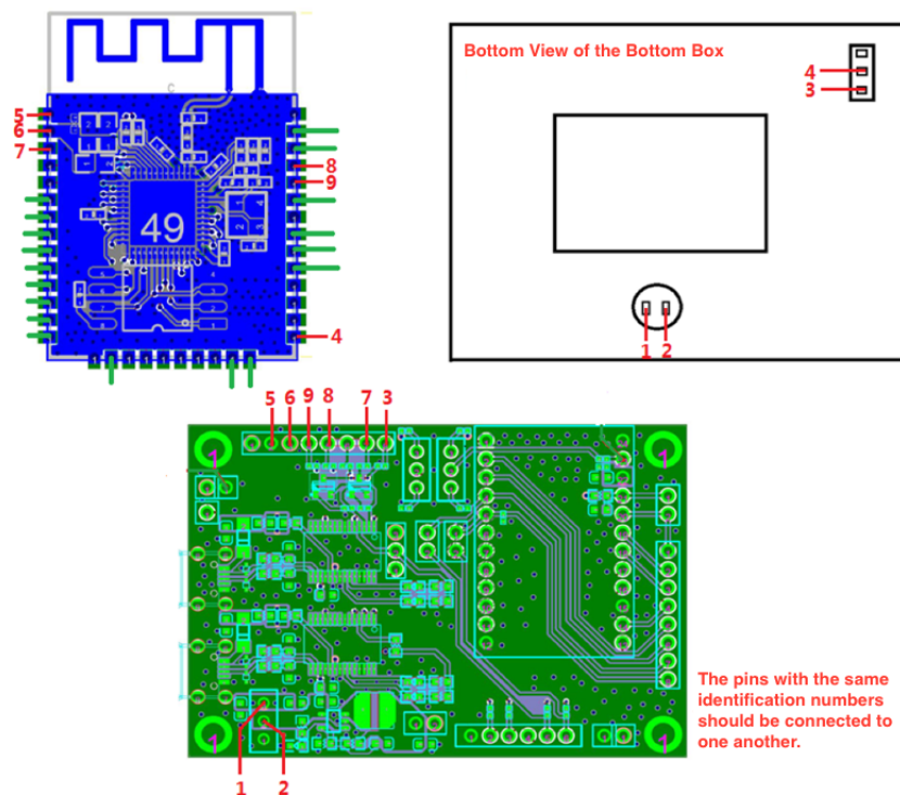
Fig. 98: The Wiring of the ESP-WROOM-32 Fixture
