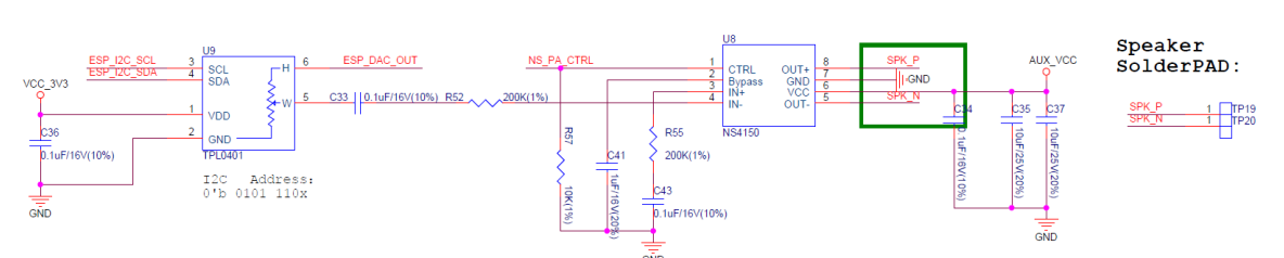
Fig. 10: ESP32-S2-HMI-DevKit-1 audio playback schematic (click to enlarge)
