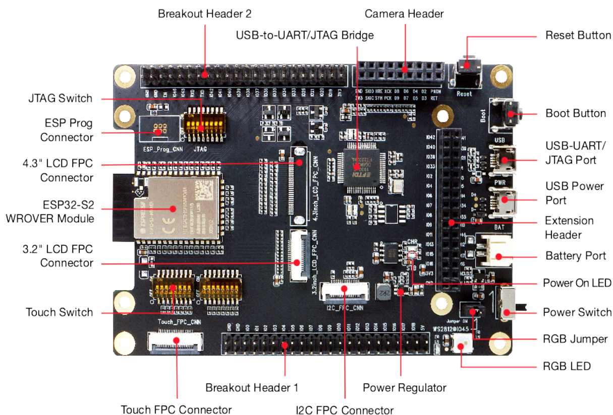
Fig. 27: ESP32-S2-Kaluga-1 - front (click to enlarge)
