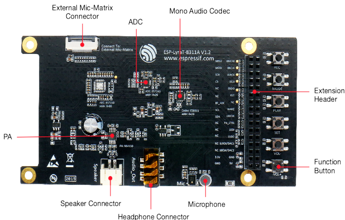
Fig. 39: ESP-LyraT-8311A - front (click to enlarge)
