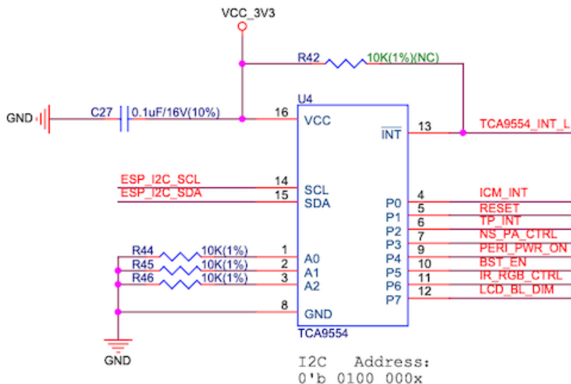
Fig. 16: ESP32-S2-HMI-DevKit-1 IO expander schematic
