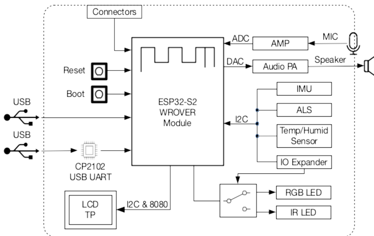
Fig. 8: ESP32-S2-HMI-DevKit-1 block diagram
