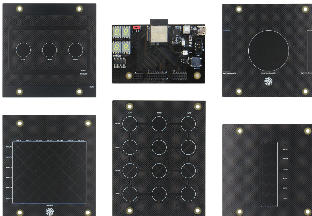
Fig. 17: ESP32-S2-Touch-Devkit-1 Board-set
