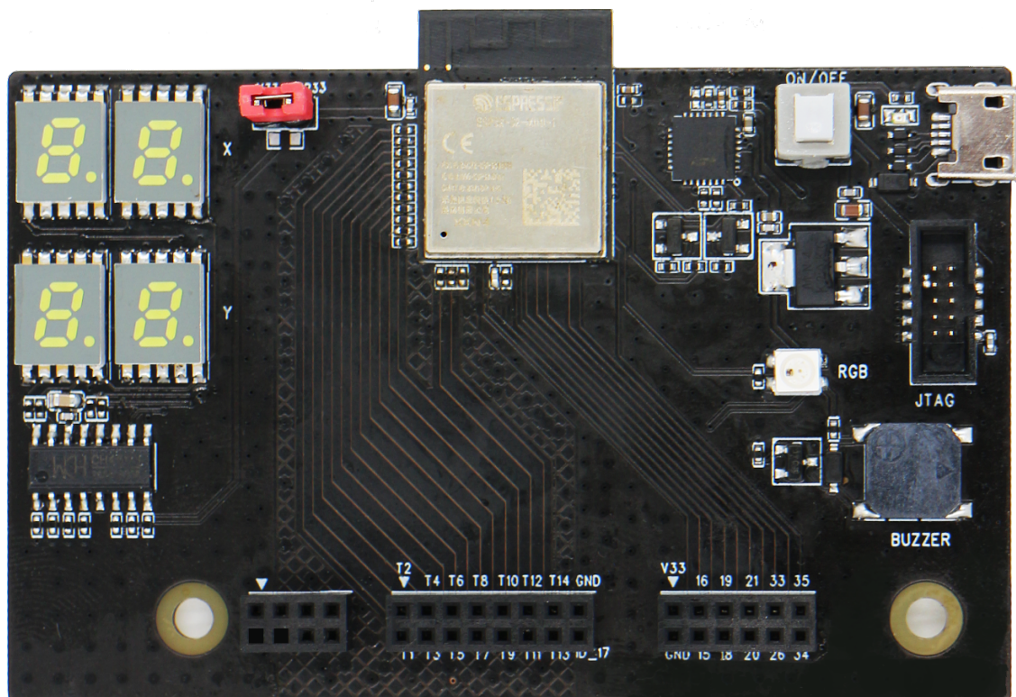
Fig. 18: Motherboard
