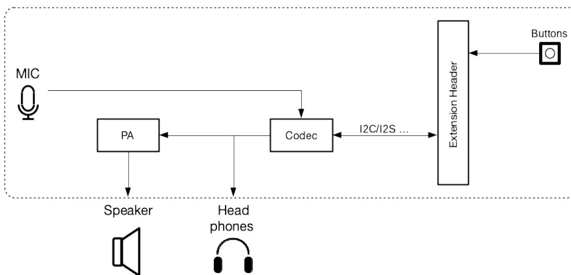
Fig. 50: ESP-LyraT-8311A block diagram
