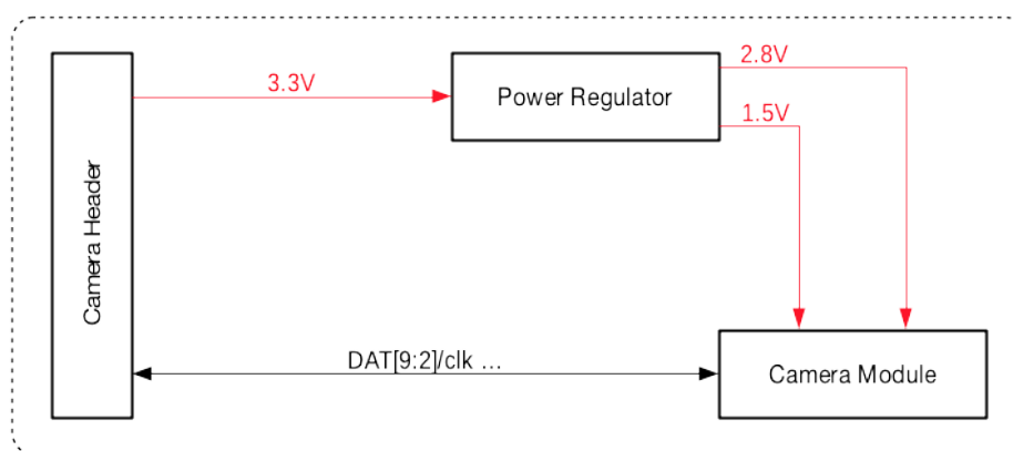
Fig. 31: ESP-LyraP-CAM block diagram
