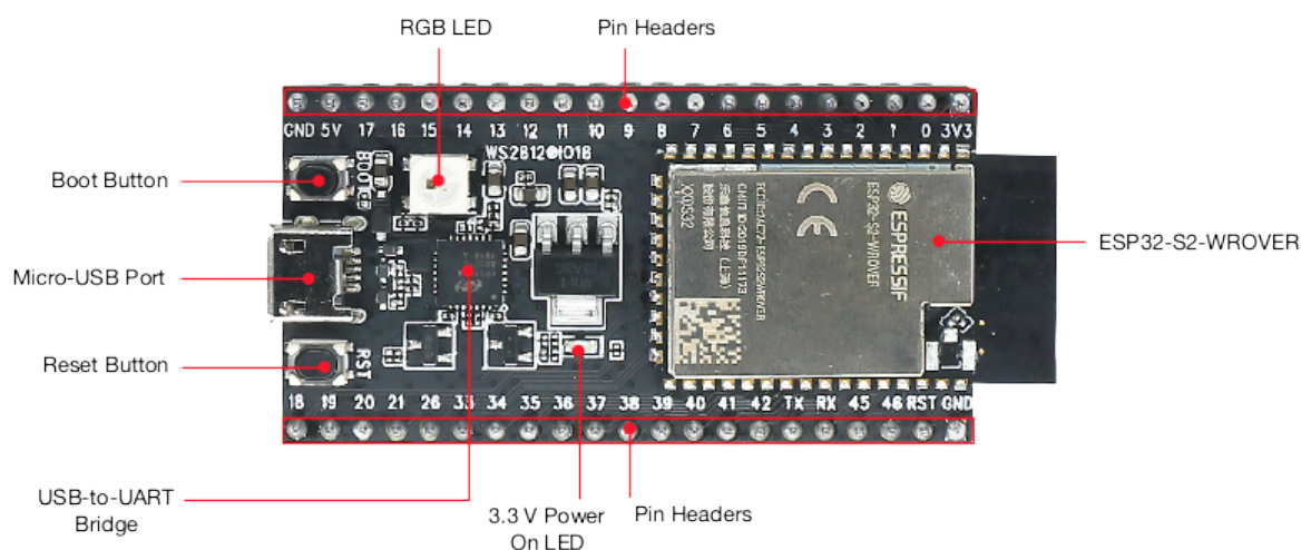
Fig. 52: ESP32-S2-Saola-1 - front
