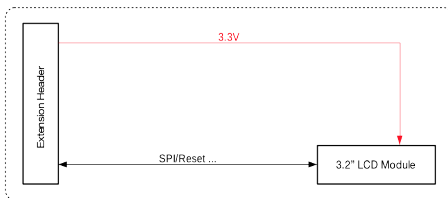
Fig. 47: ESP-LyraP-LCD32 block diagram
