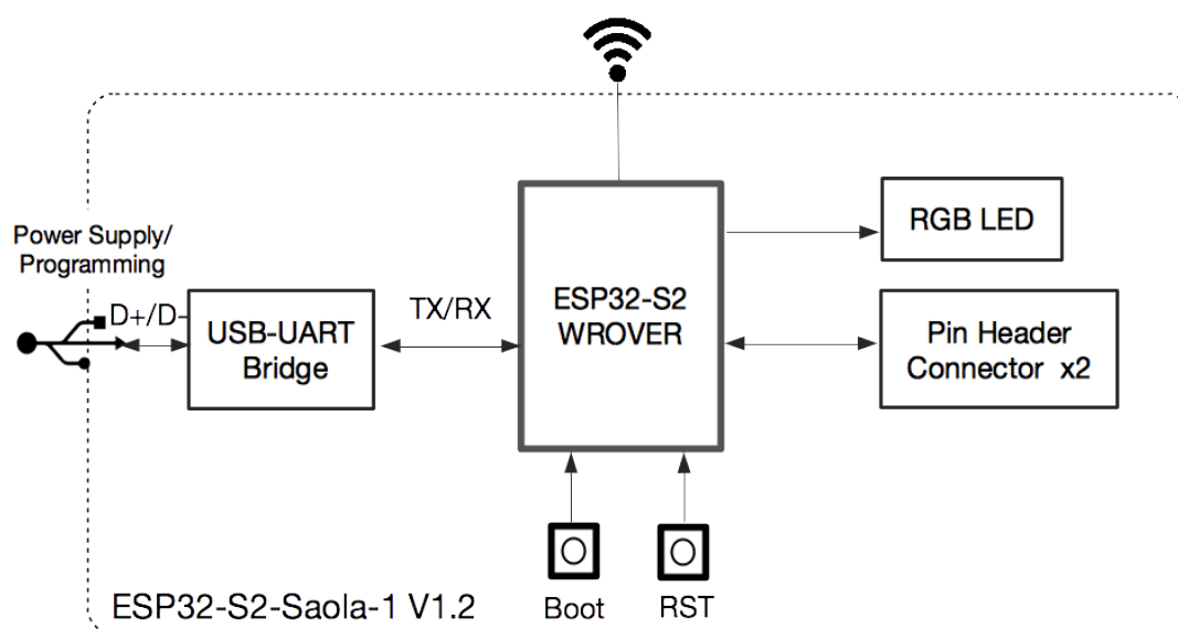
Fig. 53: ESP32-S2-Saola-1 (click to enlarge)
