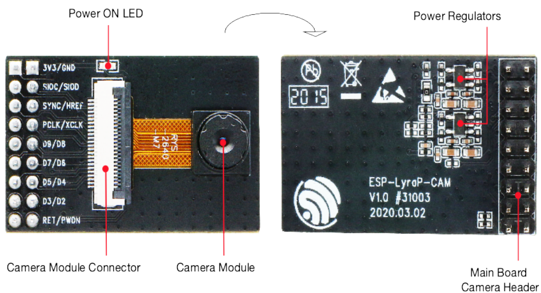
Fig. 30: ESP-LyraP-CAM - front and back
