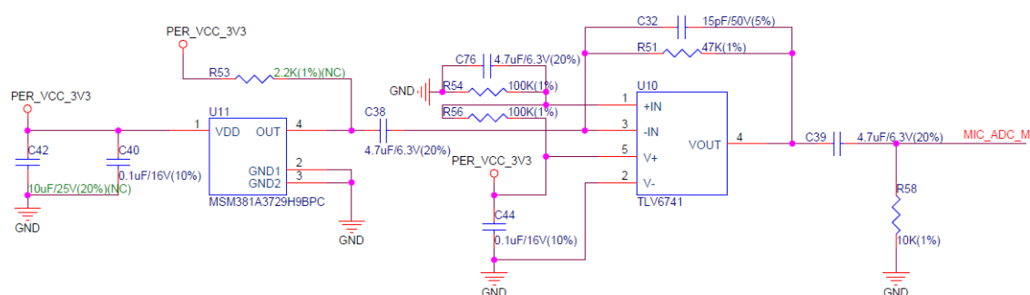
Fig. 11: ESP32-S2-HMI-DevKit-1 microphone schematic (Click to enlarge)
