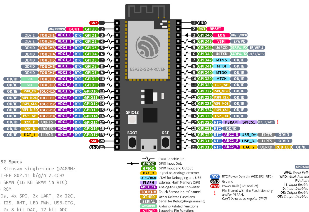
Fig. 54: ESP32-S2 Saola-1 Pin Layout (click to enlarge)
