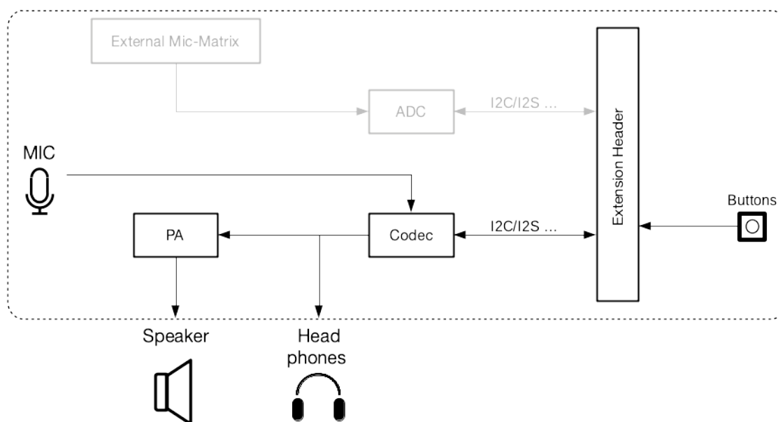
Fig. 40: ESP-LyraT-8311A block diagram
