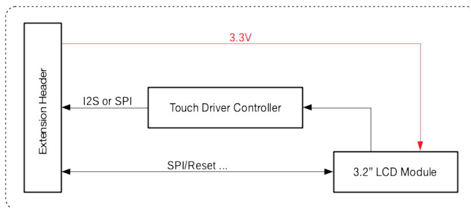
Fig. 34: ESP-LyraP-LCD32 block diagram
