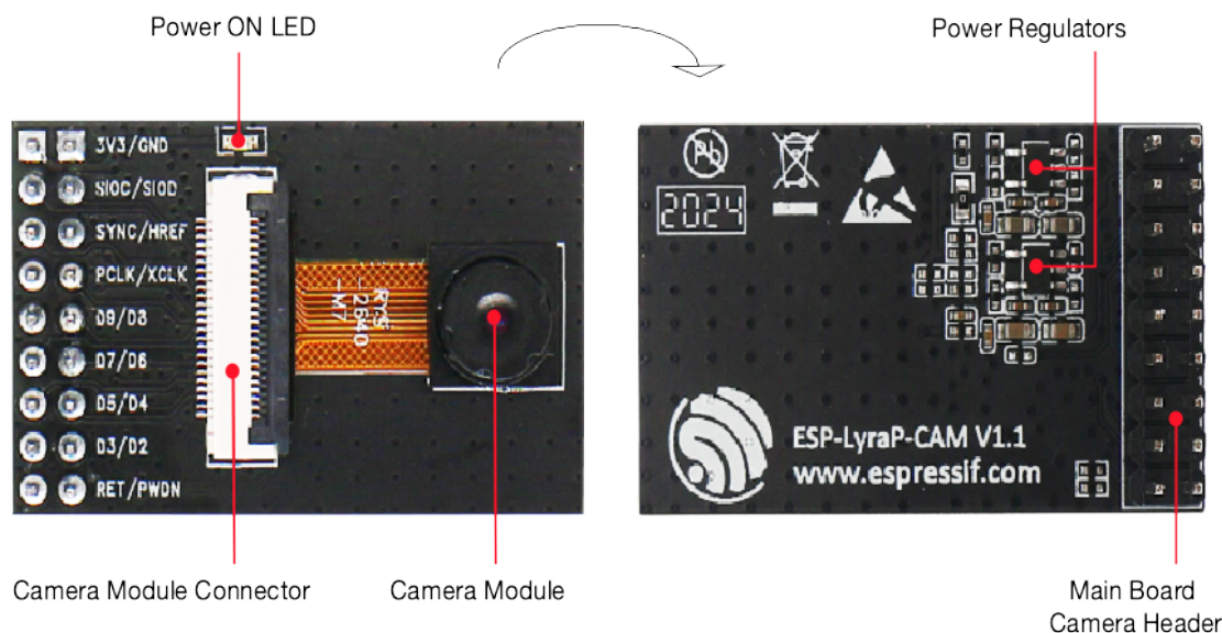
Fig. 42: ESP-LyraP-CAM - front and back
