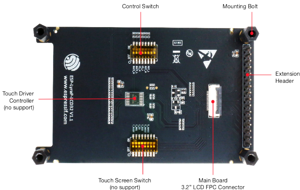
Fig. 33: ESP-LyraP-LCD32 - front (click to enlarge)
