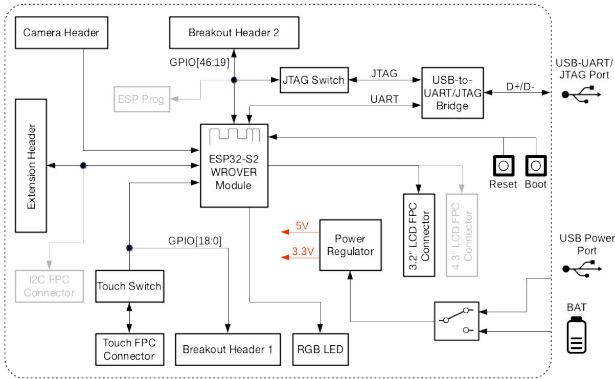
Fig. 28: ESP32-S2-Kaluga-1 block diagram
