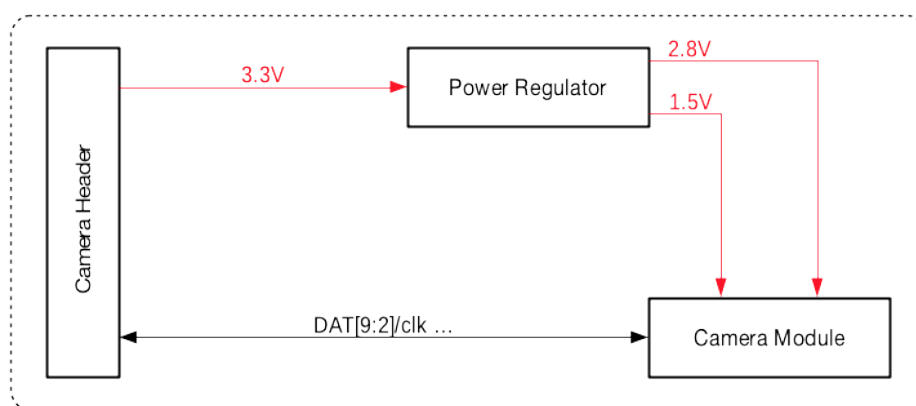
Fig. 43: ESP-LyraP-CAM block diagram
