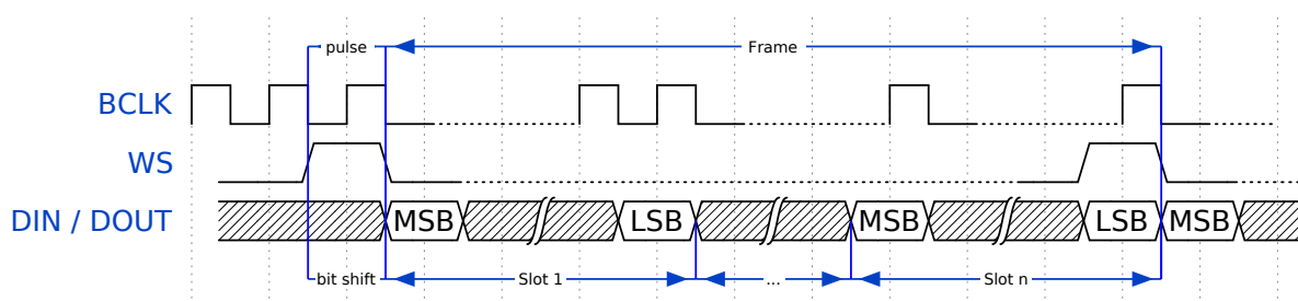
TDM PCM (short) Timing Diagram
