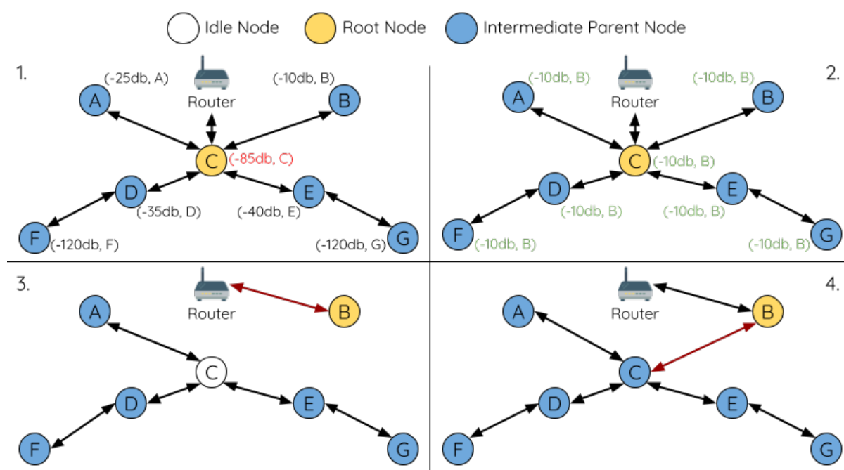
Fig. 36: Root Node Switch Example
