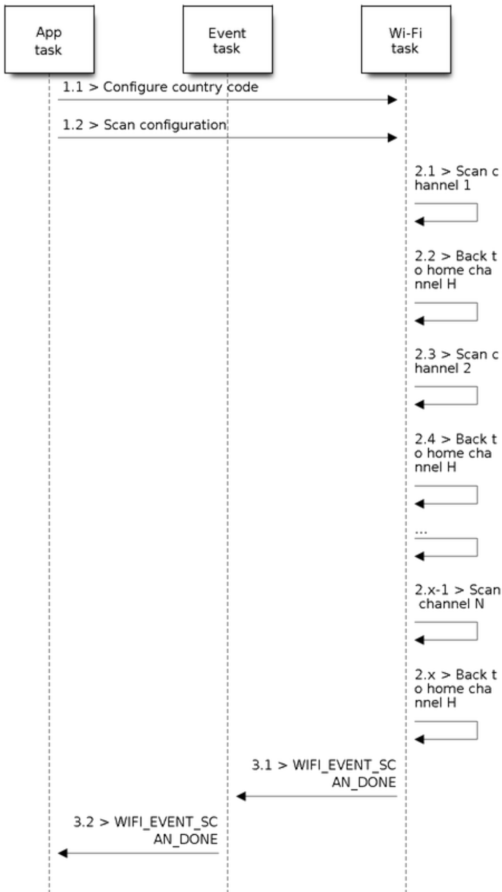
Fig. 63: Background Scan of all Wi-Fi Channels
