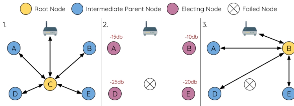
Fig. 34: Self Healing From Root Node Failure
