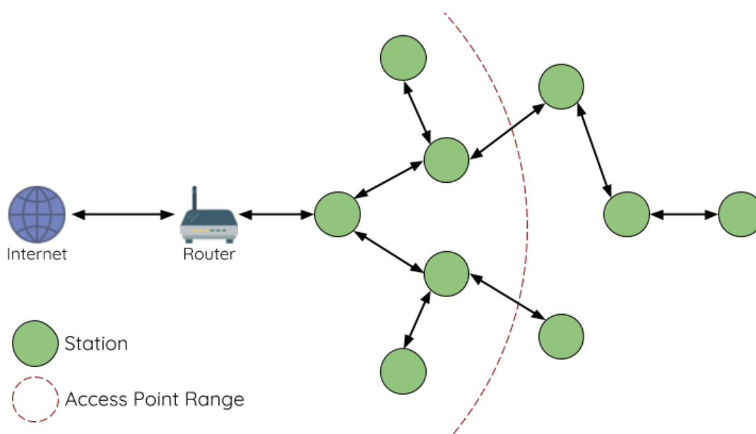
Fig. 24: ESP-WIFI-MESH Network Architecture
