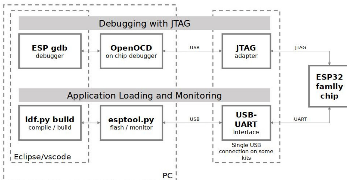
Fig. 40: JTAG debugging - overview diagram
