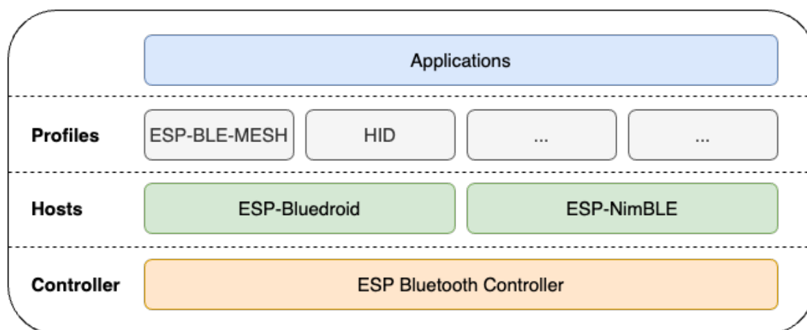
图 2: ESP32-H2 Bluetooth Stack Architecture
