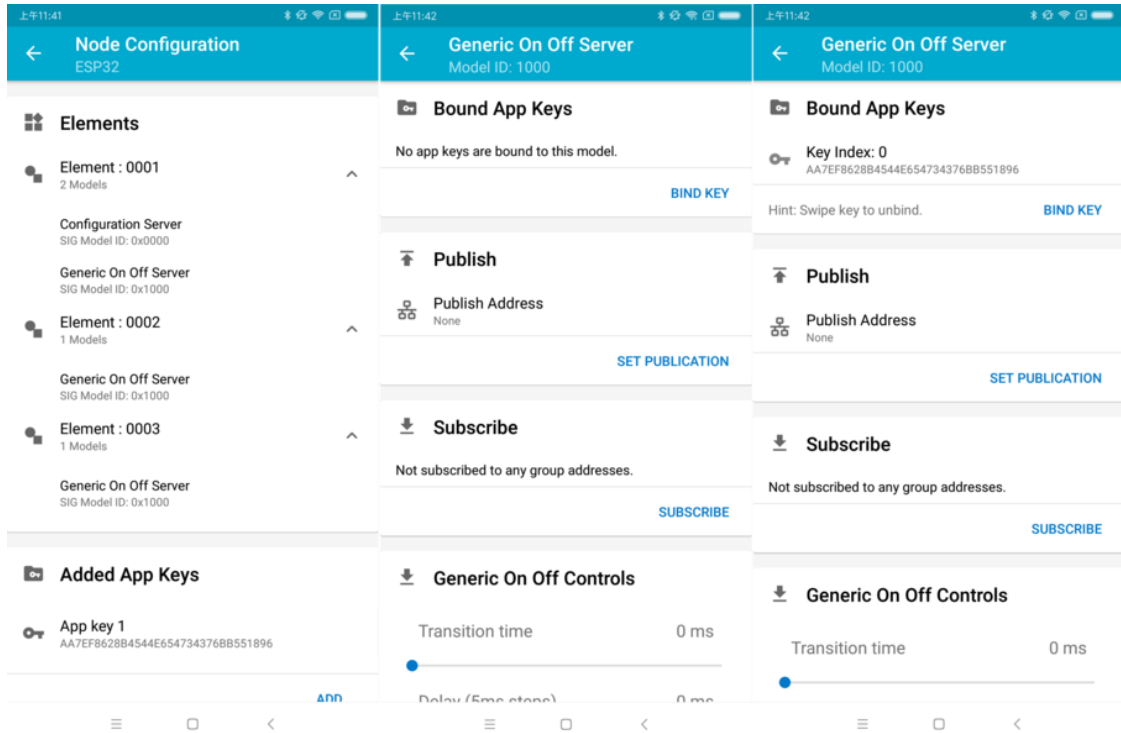
图 20: nRF Mesh - Model Bind AppKey
