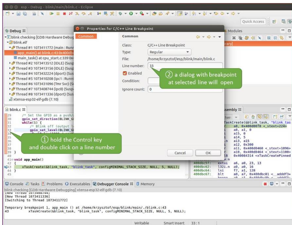
Fig. 33: Setting a breakpoint
