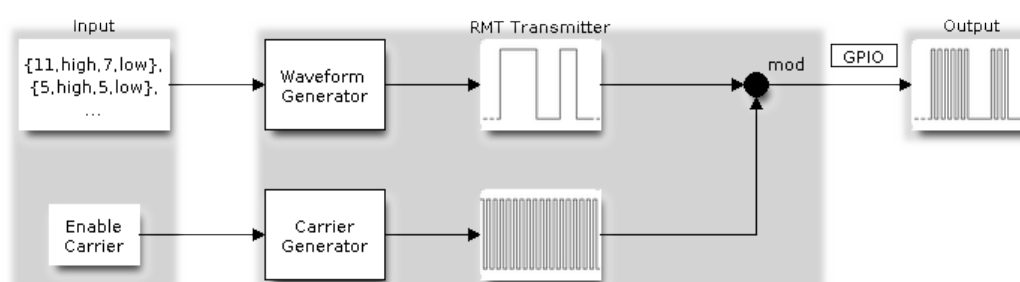
Fig. 18: Structure of RMT symbols (L - signal level)
